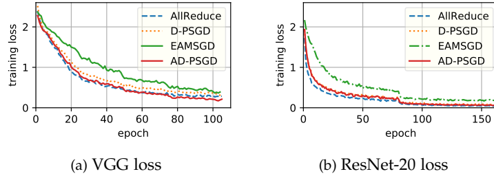
Figure 2: Training loss comparison for VGG and ResNet-20 model on CIFAR10. AllReduce-SGD, D-PSGD and AD-PSGD converge alike, EAMSGD converges the worst. 16 workers in total.
